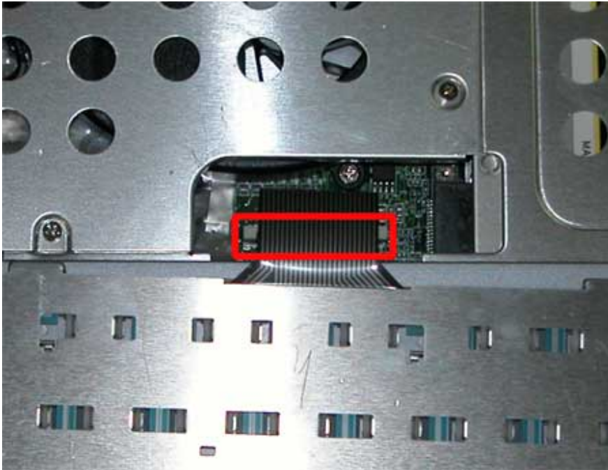
Fig. 9 Disconnecting the keyboard flat cable
